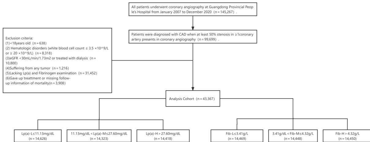
Fig. 1. Study flowchart.
