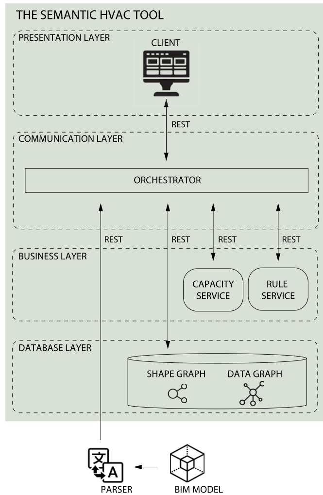
Fig. 10. The system architecture of the Semantic HVAC Tool.
