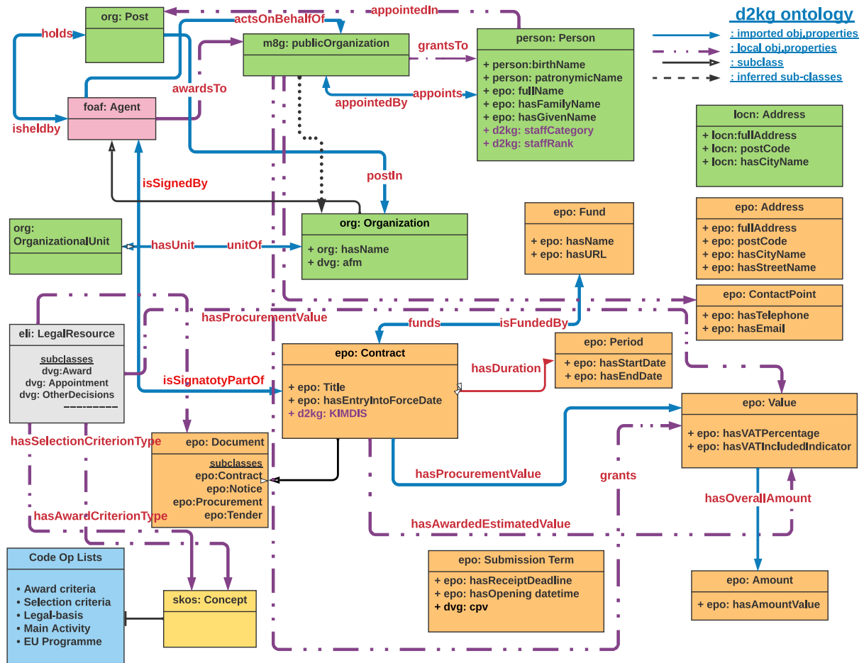
Fig. 2. Representation of the d2kg ontology.
