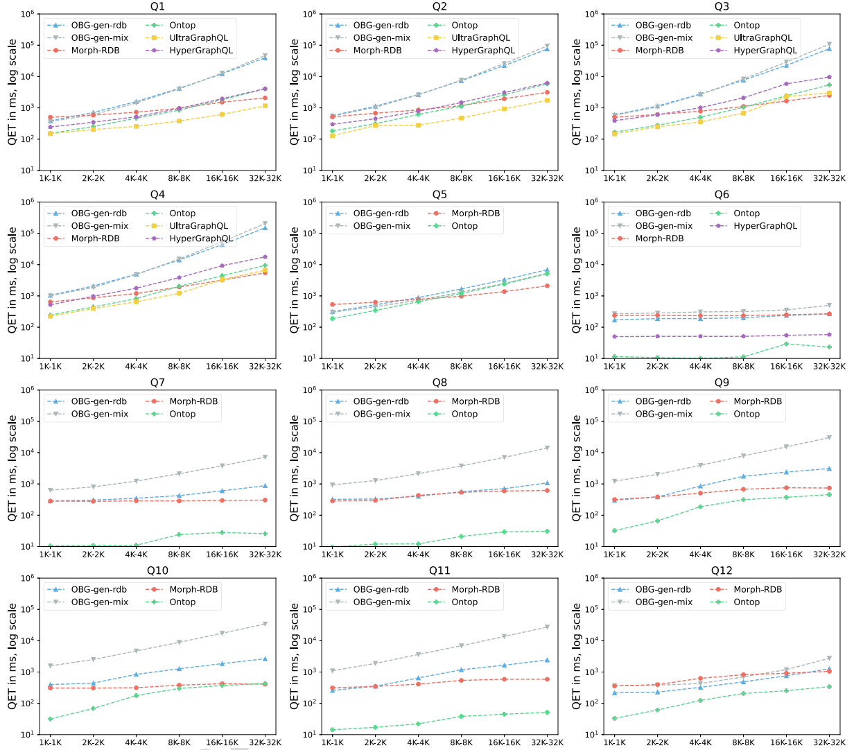
Fig. 8. Query Execution Time (QET) per query on materials dataset.
