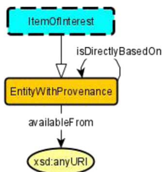
Fig. 9. A minimalistic provenance module based on the MODL Provenance pattern shown in Fig. 4.
