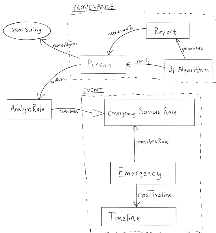
Fig. 11. Task A schema diagram.
