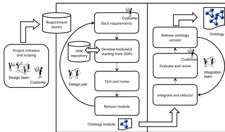
Fig. 1. eXtreme Design method overview, from [6].
