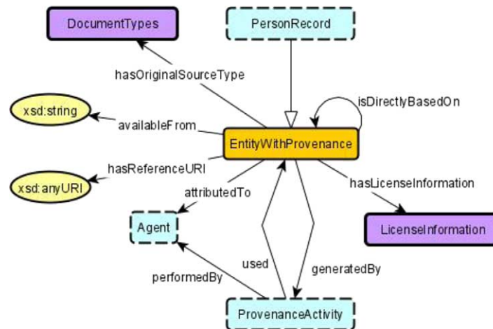
Fig. 3. Schema diagram for the Provenance module from the Enslaved Ontology [54]. It is based on the Provenance pattern from [53], which in turn is based on the core of PROV-O [44].
