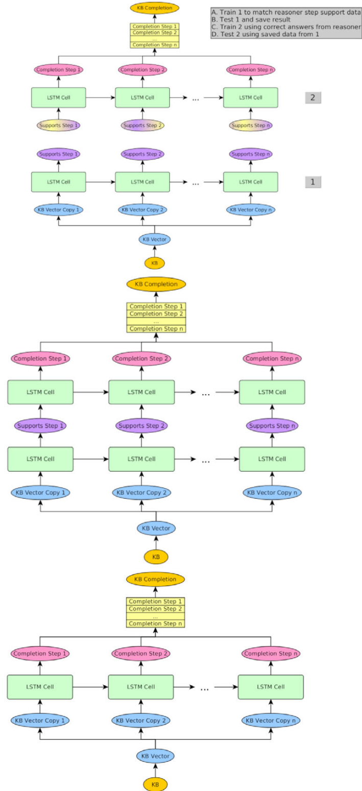
Fig. 1. Piecewise architecture (top); deep architecture (middle); flat architecture (bottom).
