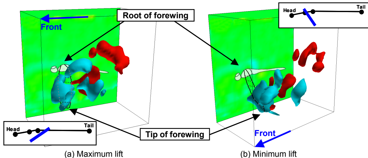
Fig. 3. Three-dimensional vortex structures around the flapping wing ( \omega / f = \pm 5 ).
