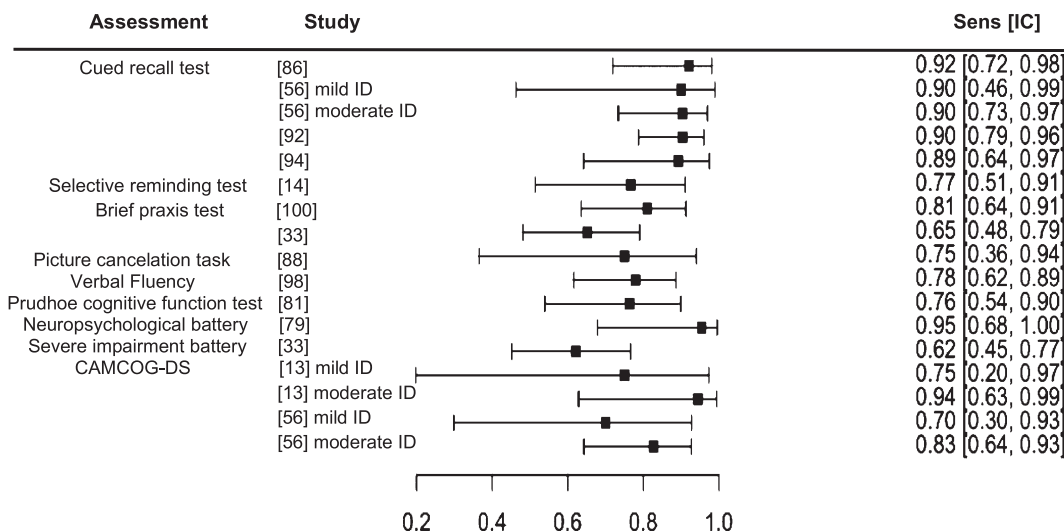
Fig. 2. Sensitivity forest plot of AD cognitive assessment.
