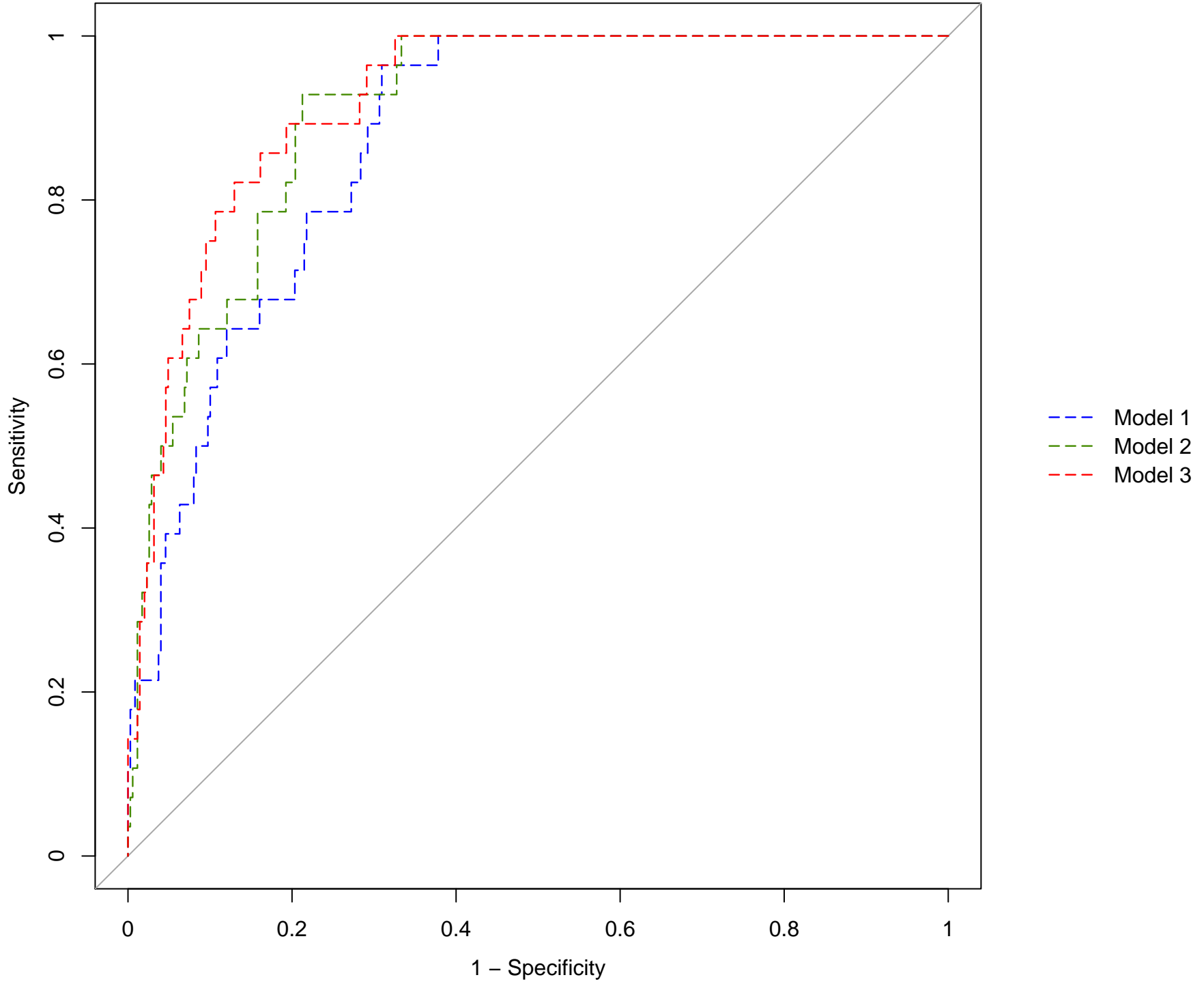
ROC curve – genetic base
