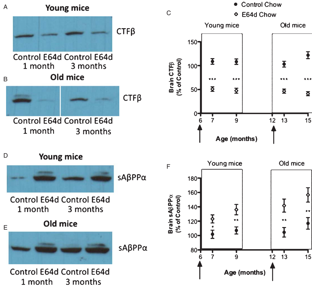
Fig. 6. Feeding E64d chow to transgenic A \beta PPLon AD mice decreases brain CTF \beta and increases sA \beta PP \alpha . Western blots show that feeding E64d chow results in qualitatively less brain CTF \beta than controls (Fig. 6A-C, arrows indicate the age at which E64d feeding began). Quantitative densitometry of the Western CTF \beta blots shows that brain CTF \beta is reduced in young and old animals fed E64d for one or 3 months by about 50% (Fig. 6C, arrows show age at which E64d chow feeding began). As CTF \beta is a proteolytic fragment of \beta -secretase cleavage, these data are consistent with E64d acting by inhibiting \beta -secretase activity. In contrast, Western blots of sA \beta PP \alpha qualitatively show that E64d feeding increased brain sA \beta PP \alpha relative to controls (Fig. 6D-F). Quantitative densitometry of the Western sA \beta PP \alpha blots shows that there is consistently more brain sA \beta PP \alpha in young and old animals fed E64d for one or 3 months than in controls (Fig. 6F). Increased sA \beta PP \alpha is consistent with E64d inhibiting \beta -secretase activity because that inhibition would allow more production of sA \beta PP \alpha . The mean and SEM are displayed at each data point (t-test comparison * p < 0.02, ** p < 0.004, *** p < 0.0001, n = 10 animals/group).
