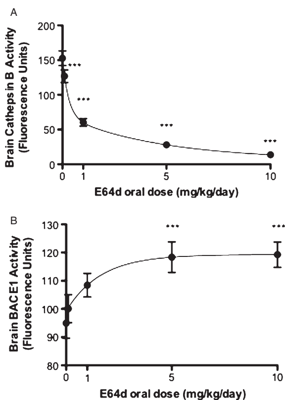
Fig. 3. E64d reduces and increases brain cathepsin B and BACE1 activities, respectively, in guinea pigs. Oral E64d administration to guinea pigs caused a biphasic dose-dependent reduction in brain cathepsin B activity with a minimum effective dose of about 1 mg/kg/day and the maximum dose lowering cathepsin B activity by 90% (Fig. 3A). As such, the brain cathepsin B effect is very similar to reduction in A \beta caused by E64d. Cathepsin B inhibition by E64d is required if the compound acts by inhibiting cathepsin B \beta -secretase activity and thus these data support that mechanism of action. In contrast, that treatment caused an increase in brain BACE1 activity with the maximum dose increasing BACE1 activity by almost 20% (Fig. 3B). The increase in BACE1 activity rules out the hypothesis that E64d reduces brain A \beta by inhibiting BACE1 \beta -secretase activity because BACE1 activity was increased. The mean and SEM are displayed at each data point (Dunnett's multiple comparison test *** p < 0.05 , n = 10 animals/group).
