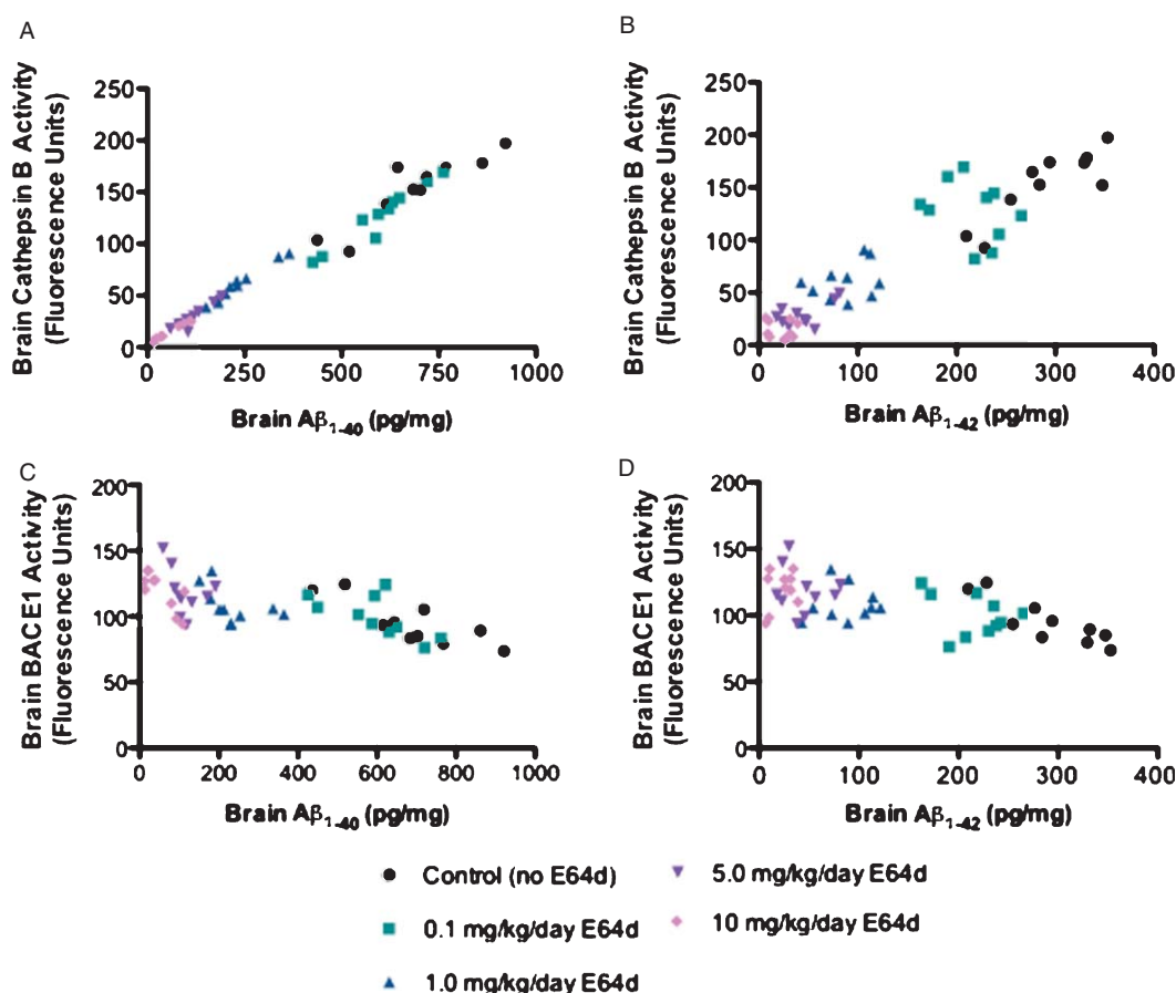
Fig. 4. Cathepsin B and A \beta are positively correlated, BACE1 and A \beta are negatively correlated in guinea pigs. The individual paired data from all guinea pigs for brain A \beta_{40} or A \beta_{42} data versus brain cathepsin B activity were plotted (Fig. 4A, B). Linear regression analysis for brain A \beta_{40} versus brain cathepsin B activity finds a r^2 = 0.98 and a 95% confidence interval for a 0.21 to 0.22 slope, which is a significantly non-zero slope at p < 0.0001 . For brain A \beta_{42} versus brain cathepsin B activity, linear regression analysis of finds a r^2 = 0.87 and a 95% confidence interval for a 0.45 to 0.56 slope, which is a significant non-zero slope at p < 0.0001 . Thus, brain cathepsin B activity is a strong predictor of brain A \beta and these data are consistent with E64d reducing brain A \beta by inhibiting cathepsin B \beta -secretase activity. In contrast, paired data from individual guinea pigs for brain A \beta_{40} or A \beta_{42} vs. brain BACE1 activity at the various E64d doses shows a very weak, slightly negative correlation (Fig. 4C, D). Linear regression analysis of brain A \beta_{40} versus brain BACE1 activity finds a r^2 = 0.45 and a 95% confidence interval for a -0.06 to -0.03 slope, which is a significant non-zero slope at p < 0.0001 . Linear regression analysis of brain A \beta_{42} versus brain BACE1 activity finds r^2 = 0.36 and a 95% confidence interval for a -0.14 to -0.06 slope, which is a significant non-zero slope at p < 0.001 . These data show that brain BACE1 activity is not predictive of brain A \beta and argue against E64d reducing brain A \beta by inhibiting BACE1 \beta -secretase activity.
