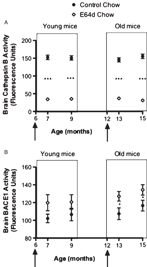
Fig. 7. Feeding E64d chow to transgenic A \beta PP/Lon AD mice reduces brain cathepsin B activity and either has no effect or increases brain BACE1 activity. Feeding E64d chow to either young or old mice for one or 3 months reduced brain cathepsin B activity by about 83% (Fig. 7A, arrows show age at which E64d chow feeding began). Brain cathepsin B inhibition is required if E64d acts by suppressing cathepsin B \beta -secretase activity and thus these data are consistent with the compound acting by that mechanism of drug action. In contrast, feeding E64d chow for one or 3 months to young mice increased brain BACE1 activity but the increase was not statistically significant (Fig. 7B). And feeding E64d chow for one or 3 months to old mice significantly increased brain BACE1 activity relative to animals feed normal chow by about 16%. These data show that the effects of E64d on brain A \beta are not due to off-target inhibition of brain BACE1 \beta -secretase activity because E64d treatment did not inhibit brain BACE1 activity, but, rather, increased brain BACE1 activity. The mean and SEM are displayed at each data point (t-test comparison *p < 0.04 , n = 10 animals/group).
