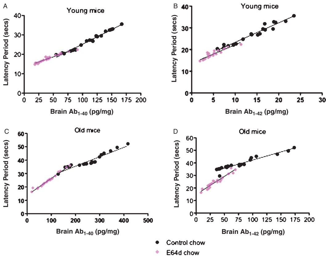
Fig. 10. Memory deficits positively correlated with brain A\beta_{40} or A\beta_{42} in transgenic A\beta PP/Lon AD mice. Paired data from individual transgenic A\beta PP/Lon mice shows that the latency period obtained in the Morris water maze test is strongly, positively correlated with brain A\beta_{40} or A\beta_{42} for control and treated young and old mice. The treated and control data combines the one and 3 month feeding schedules. In young mice, the latency period and brain A\beta_{40} is strongly positively correlated for both treated and control mice ( r^2 = 0.98 ) with similar slopes for the treated and control mice (Fig. 10A). In young mice, the latency period and brain A\beta_{42} is also strongly positively correlated for both treated and control mice ( r^2 = 0.95 ) with similar slopes for the treated and control mice (Fig. 10B). In old mice, the latency and brain A\beta_{40} is again strongly positively correlated ( r^2 = 0.95 ) but the correlation for the treated animals has a much steeper slope than that for the controls (Fig. 10C). Similarly, the old mice show a strong positive correlation between latency period and brain A\beta_{42} ( r^2 = 0.95 ) with the treated animals having a much steeper positive slope than that of the controls (Fig. 10D). These data demonstrate that memory deficits as measured by the latency period is a function of brain A\beta with more brain A\beta correlated with more memory deficits. Interestingly, the steeper correlation in the old mice for the treated animals relative to controls suggests that E64d may have other memory improving effects that are in addition to that caused by lowering brain A\beta .
