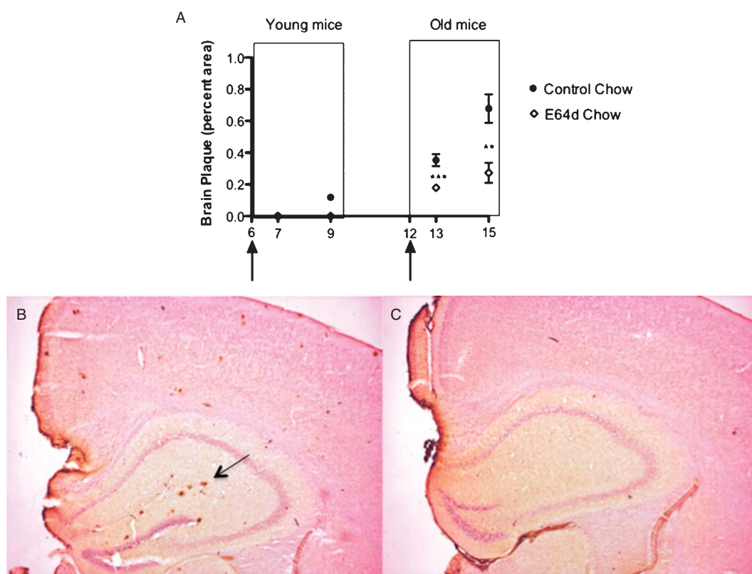
Fig. 9. E64d treatment of transgenic A \beta PPLon AD mice reduces brain amyloid plaque. Transgenic A \beta PPLon mice also mimic the pathology seen in AD patients in that they develop brain amyloid plaque as they age. Quantitative image analysis of brain sections stained for amyloid plaque in young mice show that control and treated mice have no amyloid plaque at 7 months of age and that control and E64d treated mice have very little amyloid plaque and no amyloid plaque, respectively, at 9 months of age (Fig. 9A arrows show age at which E64d chow feeding began). Quantitative image analysis of brain sections from old mice show that control mice have significant amyloid plaque at 13 and 15 months of age and that E64d significantly reduced the amyloid plaque at both ages (Fig. 9A). Histological micrographs of a brain region from a 15 month-old mouse fed control chow for 3 months shows numerous plaques, including one in the hippocampus pointed to by the arrow (Fig. 9B). A corresponding histological micrograph from a 15 month-old animal fed E64d chow for 3 months shows very little plaque (Fig. 9C). These data suggest that oral E64d administration may also be able to reduce the brain plaque seen in AD patients. The mean and SEM are displayed at each data point (t test comparison **p < 0.002 , ***p < 0.0001 , n = 10 animals/group).
