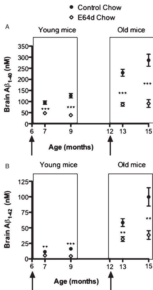
Fig. 5. Feeding E64d chow to transgenic A \beta PP23 AD mice reduces brain A \beta 40 and A \beta 42 . Brain A \beta is shown as a function of the mouse age with young (6 – 9 months of age) and old (12 – 15 months of age) mice boxed separately. The arrows indicate the age at which the experimental animals were switched from normal to E64d chow and fed that chow for either one or three months. In other words, the young animals were fed the E64d chow until they were 7 or 9 months old and the old animals were fed the E64d chow until they were 13 or 15 months old. Brain A \beta 40 was significantly reduced in both young and old mice fed either one or three months (Fig. 5A, arrows indicate age at which E64d feeding began, and Table 1). Brain A \beta 42 was also significantly reduced in both young and old mice fed E64d chow for either one or three months (Fig. 5B and Table 2). Thus, even though brain A \beta 40 and A \beta 42 increased with increasing age in control animals, the A \beta 40 and A \beta 42 in the E64d treated animals was consistently reduced at both ages and feeding schedules. Particularly significant is that E64d was efficacious at reducing A \beta 40 and A \beta 42 in the old animals even though feeding was not initiated until after those animals had accumulated abnormal levels of A \beta 40 and A \beta 42 . This suggests that the compound is effective at arresting further brain A \beta 40 and A \beta 42 accumulation even after abnormal levels have developed. The mean and SEM are displayed at each data point. Stars represent statistically significant differences between the means of age-matched E64d and normal chow fed mice (t-test comparison *** p < n = 10 animals/group).
