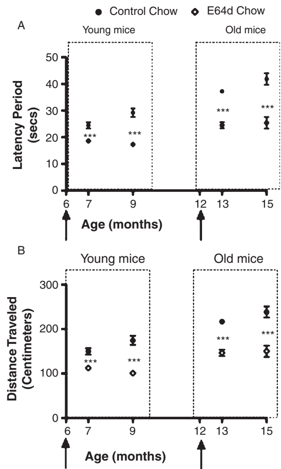
Fig. 8. Feeding E64d chow to transgenic A \beta PP/Lon AD mice improves memory deficits and memory retention. As they age, transgenic A \beta PP/Lon mice mimic the behavior of AD patients in that they progressively develop memory deficits, which can be assessed using the Morris water maze test by measuring the time it takes the animals to find a invisible, submerged platform (latency period) and distance traveled to find that platform. Feeding E64d chow to young ((6–9 months) or old (12–15 months of age) mice for either one or 3 months significantly improved the animals' ability to remember the location of the platform as measured by the latency period (Fig. 8A, arrows indicate age at which E64d feeding began, and Table 3). Significantly, E64d treatment improved memory deficits in 15-month-old animals, which had significant memory deficits, suggesting that the compound may be able to restore memory after a deficit has occurred. Similarly, feeding E64d chow to young or old mice for either one or 3 months reduced the distance traveled (Fig. 8B and Table 4) Again, this data shows that oral administration of E64d is able to improve memory deficits that otherwise will occur in this transgenic AD animal model. To test memory retention, mice were also tested for the percentage of time spent in the northeast (NE) target quadrant after the platform was removed from that quadrant (Fig. 8C and Table 5). All E64d treated groups spent more time in the target quadrant than did age-matched untreated animals showing that the E64d resulted in greater memory retention. Together, these data suggest that oral E64d administration may also be able to prevent or reverse the memory decline seen in AD patients. The mean and SEM are displayed at each data point (t test comparison ***p < 0.0001 , n = 10 animals/group).
