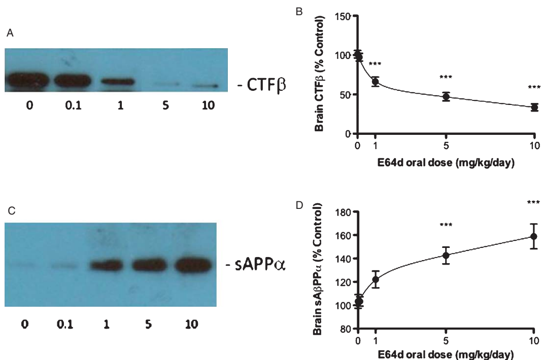
Fig. 2. E64d lowers and increases brain CTF \beta and sA \beta PP \alpha , respectively, in guinea pigs. Oral administration of E64d to guinea pigs caused a dose-dependent reduction in brain CTF \beta with the maximum dose reducing CTF \beta by more than 50% (Fig. 2A, B). CTF \beta is a proteolytic product of \beta -secretase cleavage of A \beta PP and thus these data are also consistent with the compound acting by inhibiting \beta -secretase activity. In contrast, the oral E64d treatment caused a dose-dependent increase in brain sA \beta PP \alpha with the maximum dose increasing sA \beta PP \alpha by about 54% (Fig. 2C, D). These data are consistent with E64d inhibiting \beta -secretase activity because sA \beta PP \alpha is derived from A \beta PP \alpha -secretase cleavage, which competes with \beta -secretase cleavage of A \beta PP, and thus the inhibition of \beta -secretase activity provides more A \beta PP for \alpha -secretase to produce more sA \beta PP \alpha . The mean and SEM are displayed at each data point (Dunnett's multiple comparison test *** p < 0.05, n = 10 animals/group).
