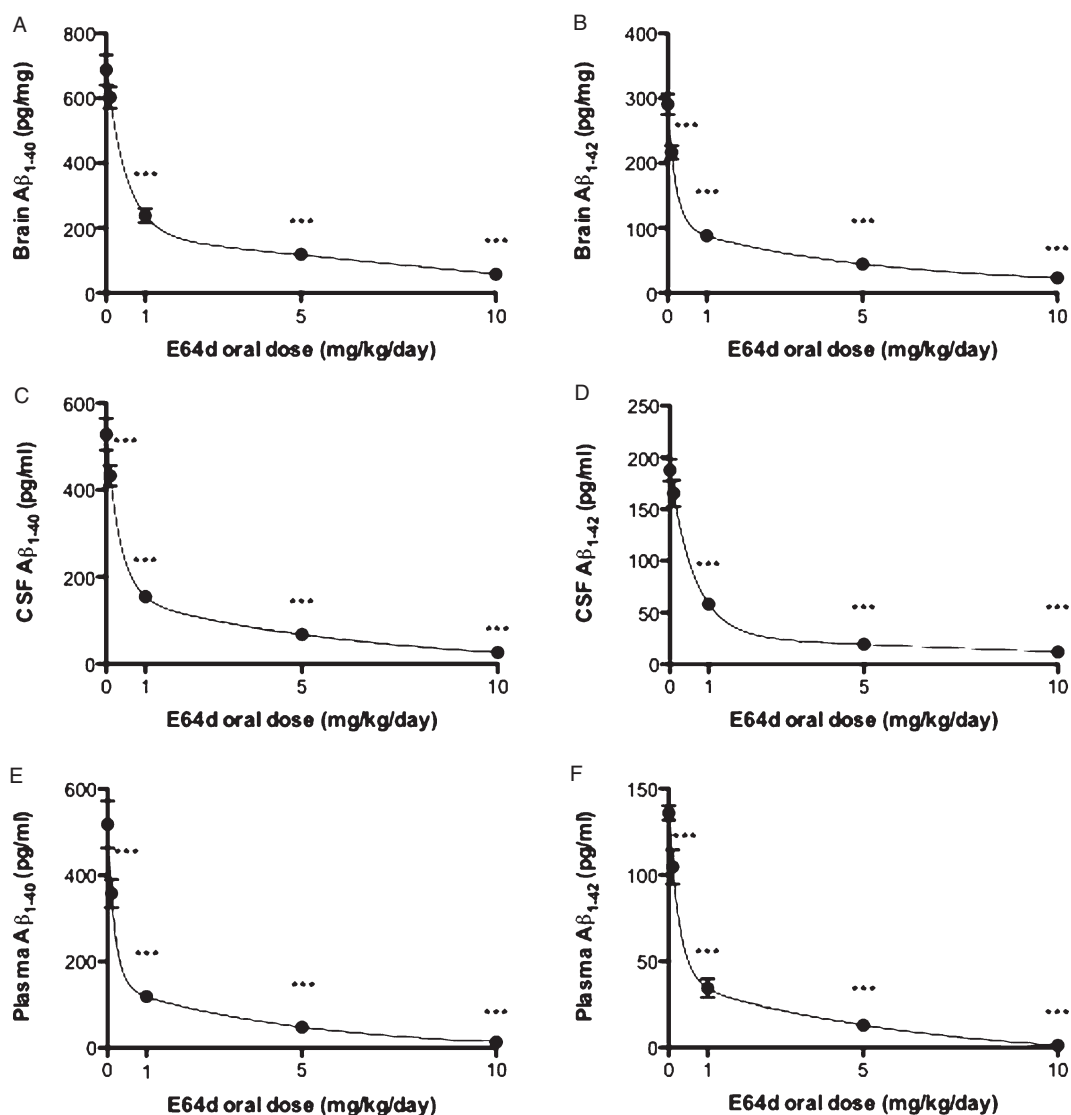
Fig. 1. E64d reduces brain, CSF, and plasma Aβ 40 and Aβ 42 in guinea pigs. Once-a-day oral administration of E64d for one week to guinea pigs results in similar biphasic dose-dependent reductions in (A) brain Aβ 40 , (B) brain Aβ 42 , (C) CSF Aβ 40 , (D) CSF Aβ 42 , (E) plasma Aβ 40 , and (F) plasma Aβ 42 . The minimum effective dose was about 1 mg/kg/day. The maximum dose (10 mg/kg/day) caused a 90% reduction or more in both Aβ 40 and Aβ 42 in all compartments. The guinea pig is a natural model of human wild-type AβPP processing and, thus, the major reduction in Aβ caused by oral E64d administration in that model suggests that the compound may have similar effects in humans. The fact that both Aβ 40 and Aβ 42 were similarly affected in all compartments is consistent with the compound inhibiting β-secretase production of Aβ. The mean and standard error of the mean (SEM) are displayed at each data point. For some data points, the error bars are smaller than the symbol representing the mean and, therefore, the error bars are not visible. Stars represent those E64d dose groups, which are statistically different from the control group (no E64d) (Dunnett's multiple comparison t-test *** p < 0.05, n = 10 animals/group).
