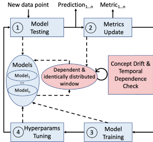
Fig. 6. Proposed architecture to manage concept drift and temporal dependence.
