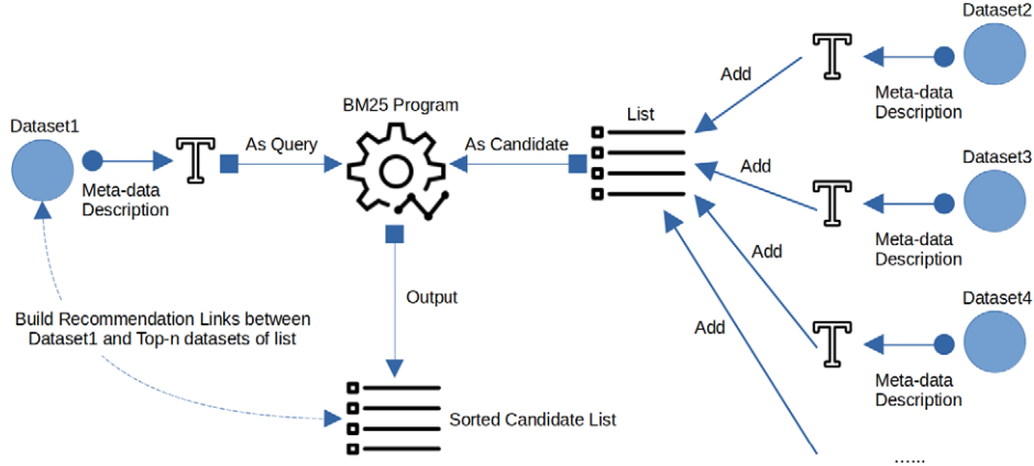
Fig. 3. Dataset recommendation based on BM25.
