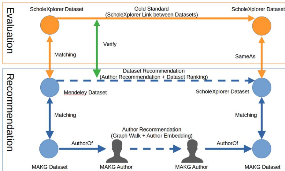
Fig. 4. The overview of dataset recommendation and evaluation in our experiments.
