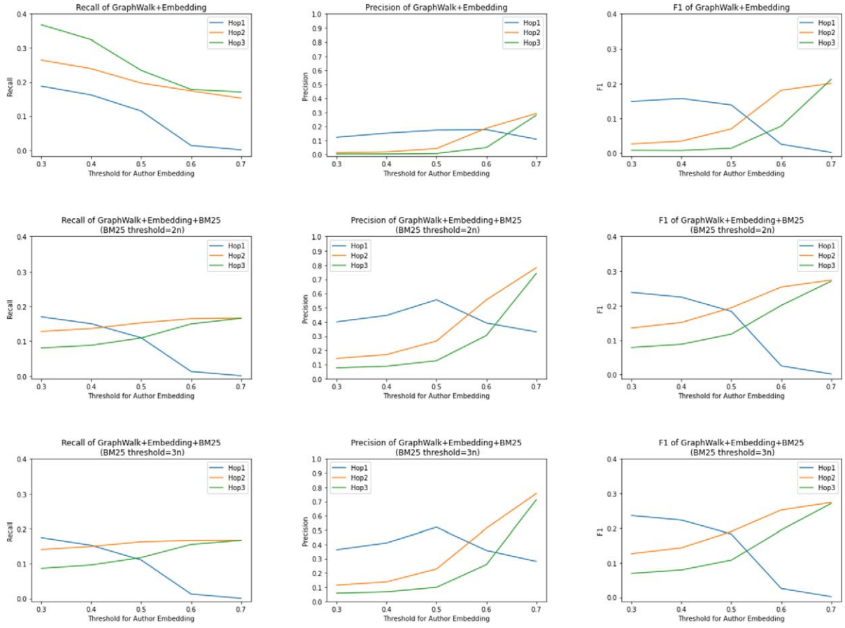
Fig. 6. Recall (column 1), precision (column 2) and F1 score (column 3) for GW&AE experiment (row 1), GW&AE + DRank experiment with T_{BM25} = 2n (row 2) and GW&AE + DRank experiment with T_{BM25} = 3n (row 3).
