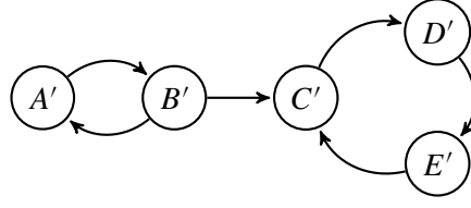
Fig. 4. Argumentation framework AF_{P_{AF_2}} .
