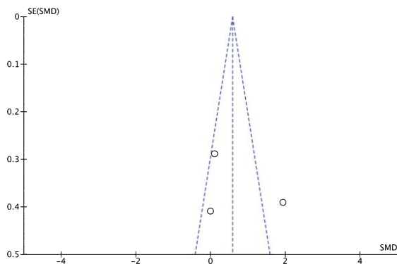
Fig. 3. To visually assess for publication bias, a funnel plot of the three studies included in the quantitative analysis has been prepared. However, since the plot is balanced with a wide range in study results (Kendall's Tau = 0.3333, p = 1.0000 ), it appears that the risk of publication bias in this case is small. The Fail-Safe N was calculated to be 8 using the Rosenthal approach.
