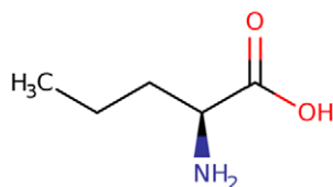
Fig. 5. The class L-2-aminopentanoic acid , which had been wrongly axiomatised as a subclass of nitrile (which has now been corrected in ChEBI). It does not feature the required triple bond but a chiral structure in its place.
