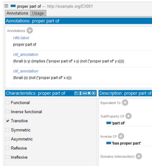
Fig. 1. View of an annotated OWL entity in Protégé.
