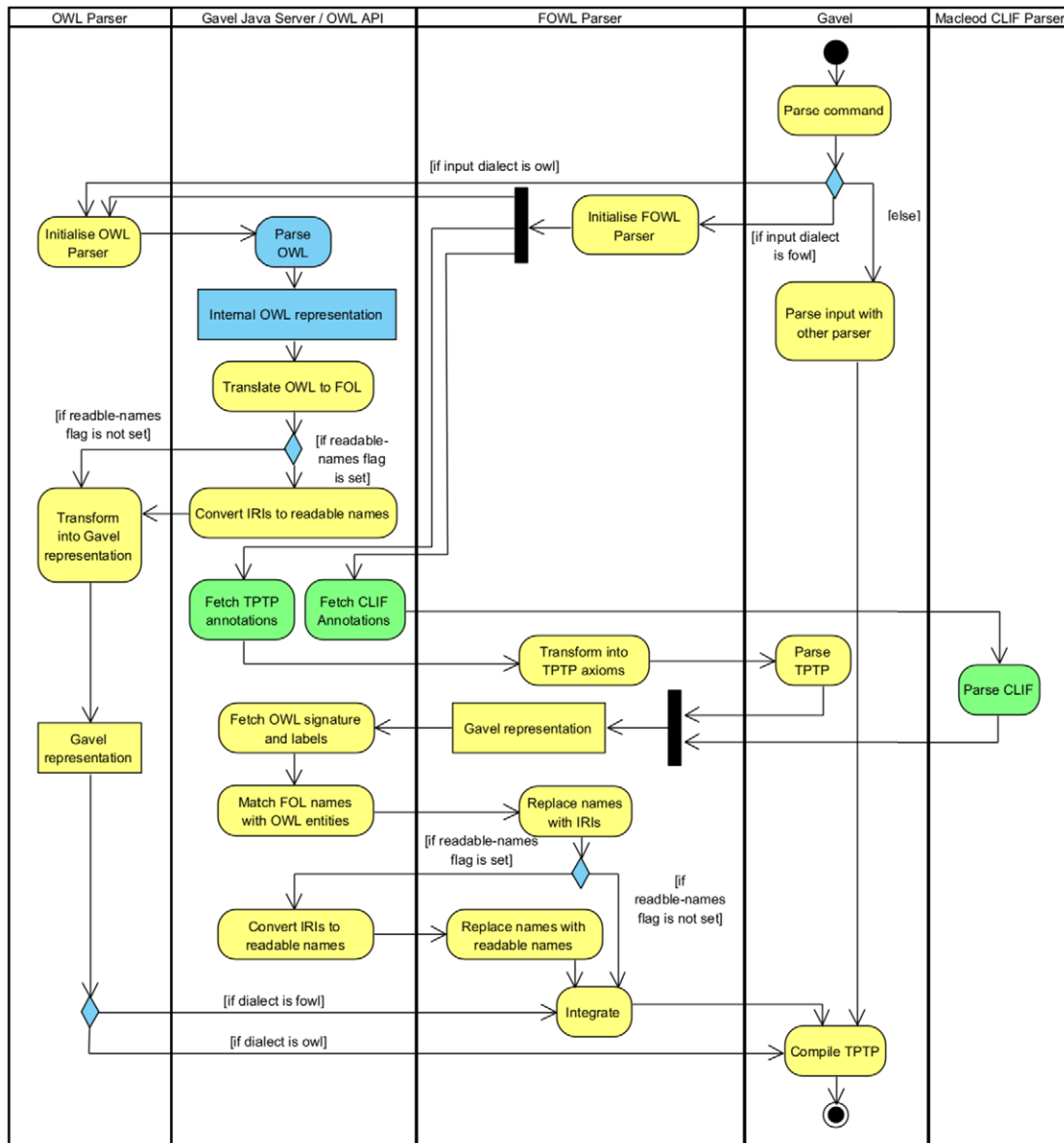
Fig. 2. A UML activity diagram illustrating the process of translating an annotated OWL ontology or standard OWL ontology into TPTP. Actions that were newly implemented for the translation tasks are shown in yellow, actions that were reused from existing tools are marked in blue. For green actions, the existing functionality has been extended.
