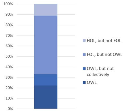
Fig. 3. The shares of KGEMT axioms which can be represented in OWL, FOL and HOL respectively.
