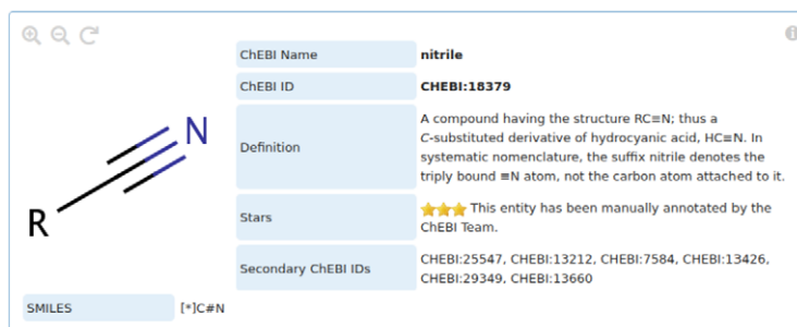
Fig. 4. The class nitrile as represented on the ChEBI website. The SMILES string [*]C#N specifies a molecule that contains a carbon atom (C) that is connected to nitrogen (N) via a triple bond (#) and some unspecified structure (*).
