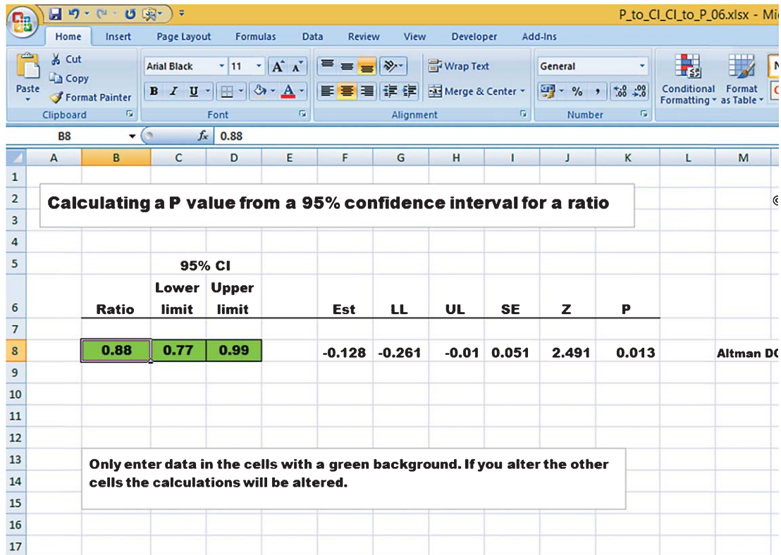
Fig. 3. Screen shot for calculating a P value from a 95% CI for a ratio.
