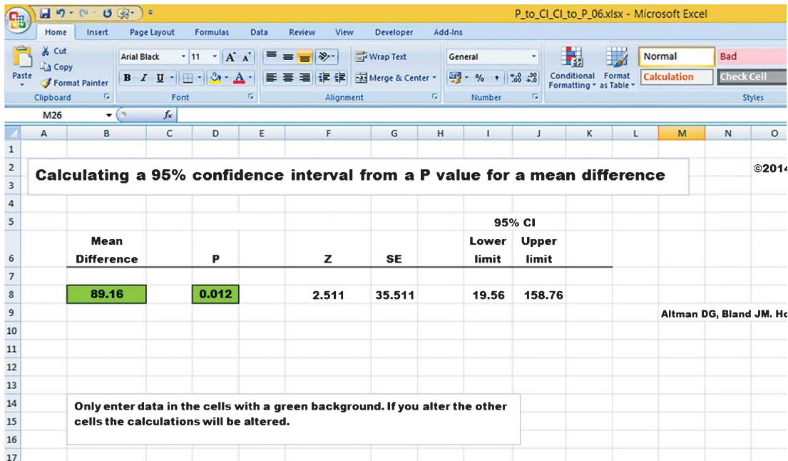
Fig. 2. Screen shot for calculating a 95% CI from a P value.
