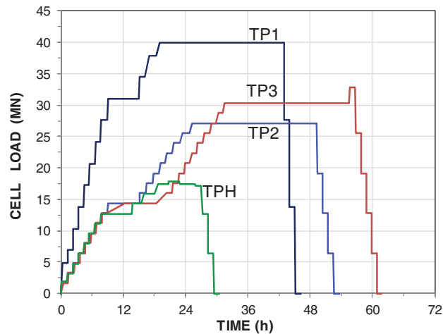
Fig. 6. Loading schedule for the test piles.
