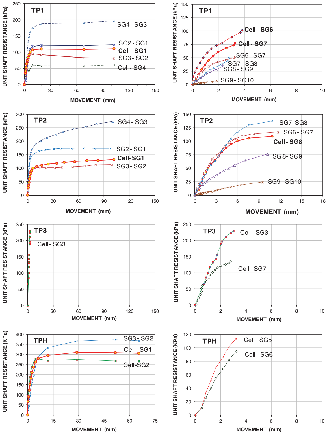
Fig. 12. Unit shaft resistances.
