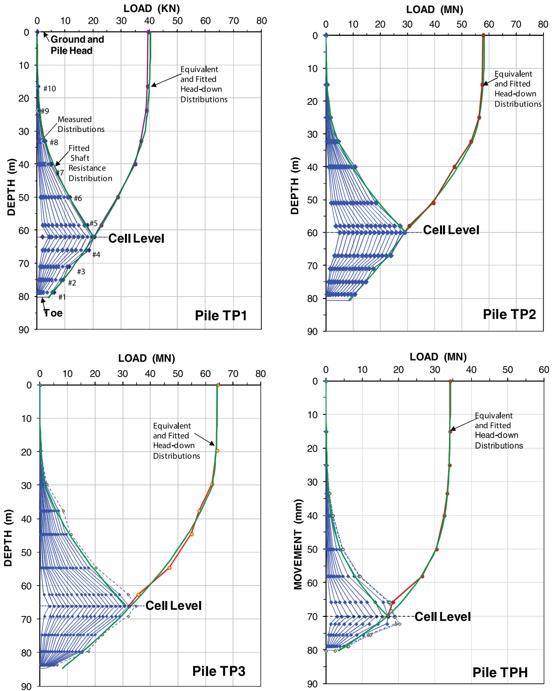
Fig. 10. Load distributions: Measured and fitted in effective stress analysis.
