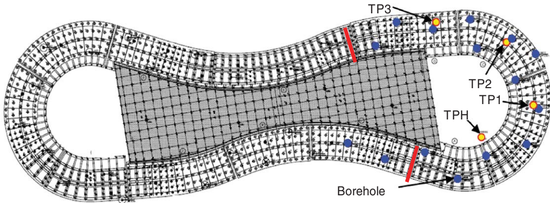
Fig. 3. Layout of test piles and Boreholes in phase 1.
