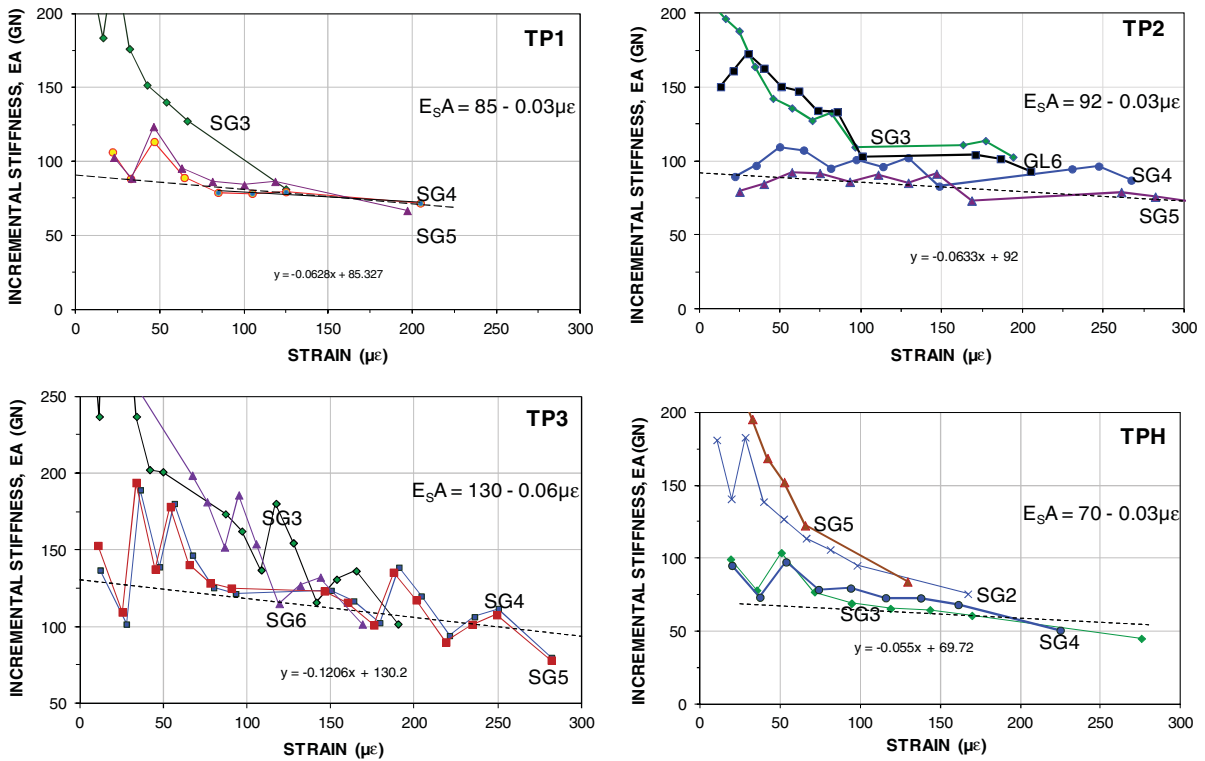
Fig. 9. Incremental stiffness plots with approximate secant stiffness values.
