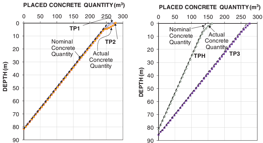
Fig. 5. Nominal and as-placed concrete volumes.
