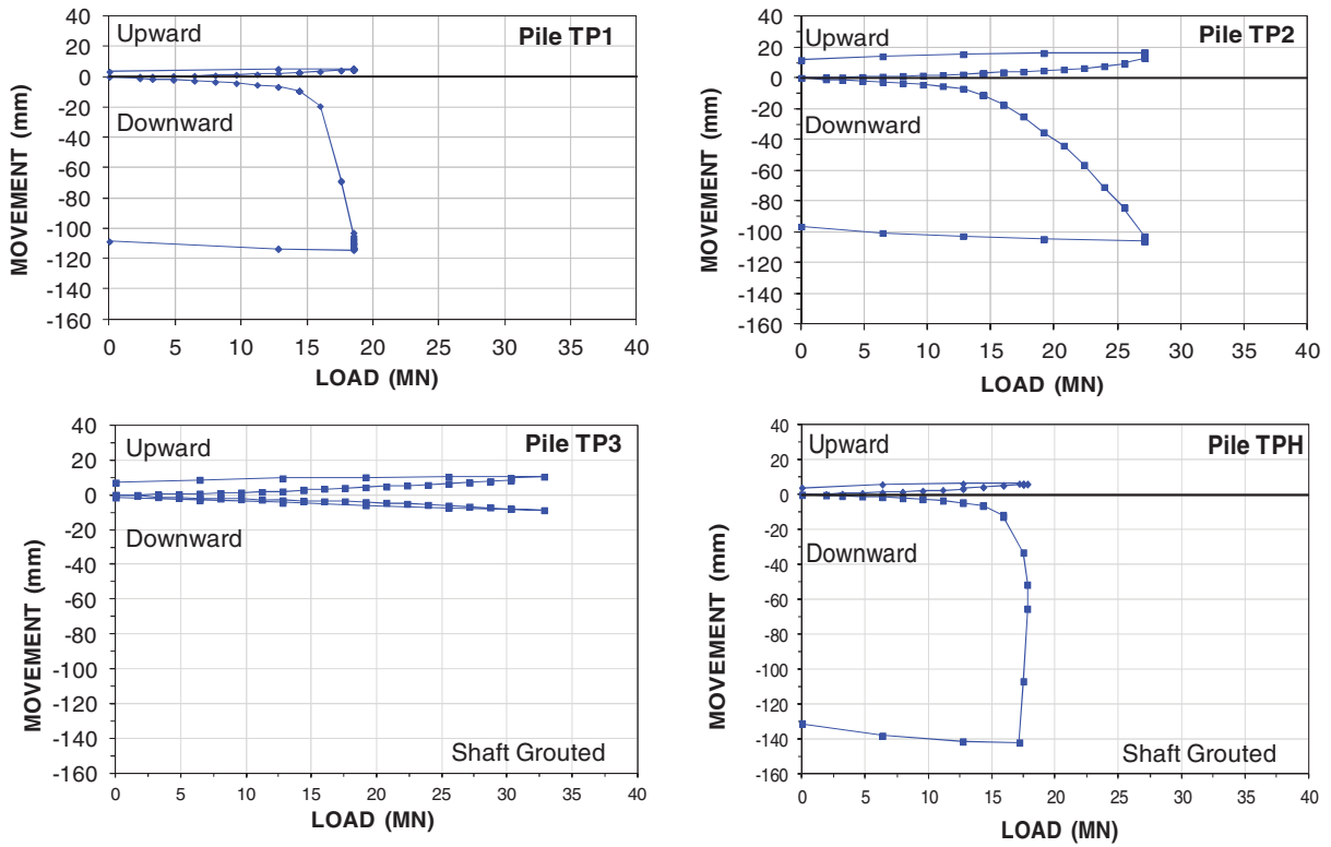
Fig. 7. Upward and downward load-movement curves.
