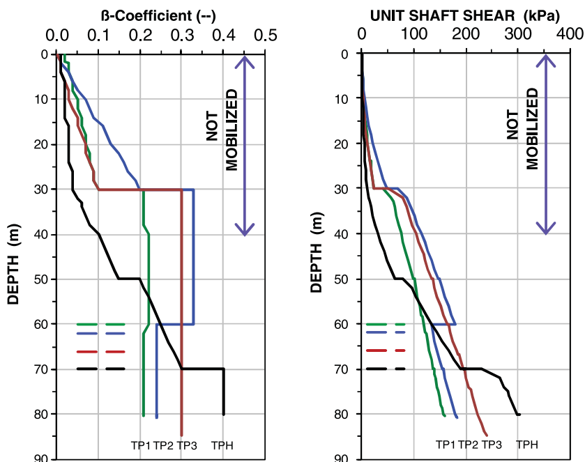
Fig. 11. Distributions of beta-coefficients and unit shaft shear.
