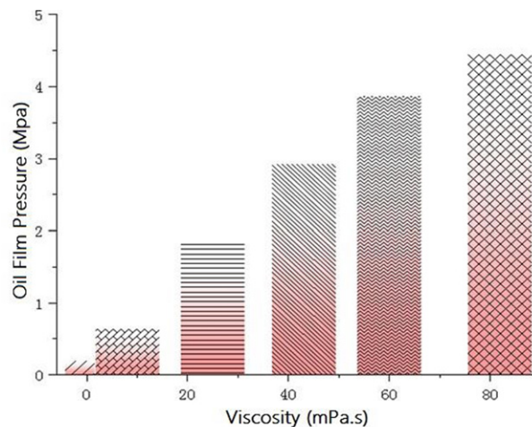
Fig. 15. Oil film pressure distribution at different viscosities.
