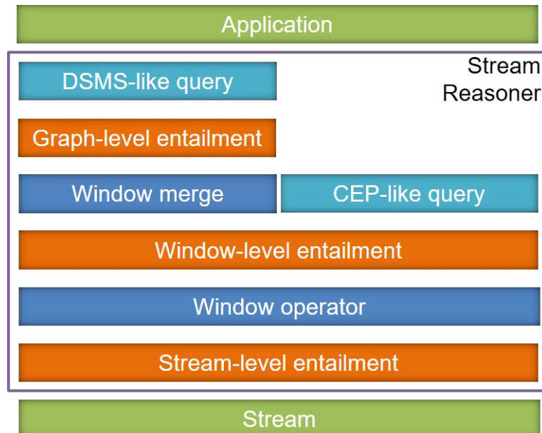
Fig. 1. A model to describe stream reasoners.
